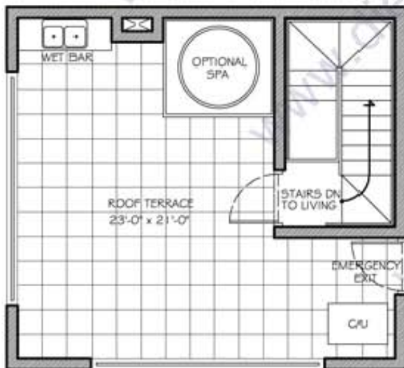
ROOF TERRACE
