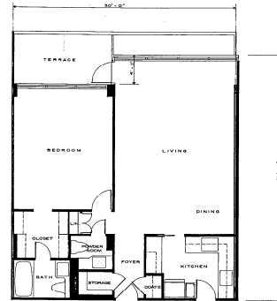
FLOOR PLAN - APARTMENT 03 ONE BEDRM., 1/2 BATH, TERRACE 1,000 SQ. FT. FLOOR NO
