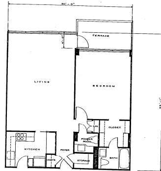
FLOOR PLAN - APARTMENT 02, 06, 10, 16. ONE BEDROOM, BATH, TERRACE 1,000 SQ. FT. FLOOR NO
