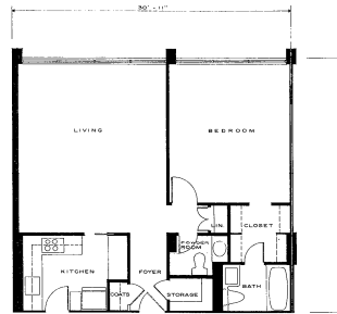
FLOOR PLAN - APARTMENT 101
