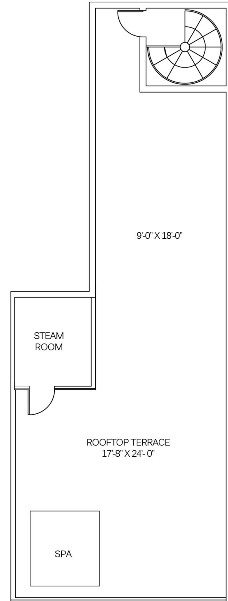
ROOFTOP TERRACE
